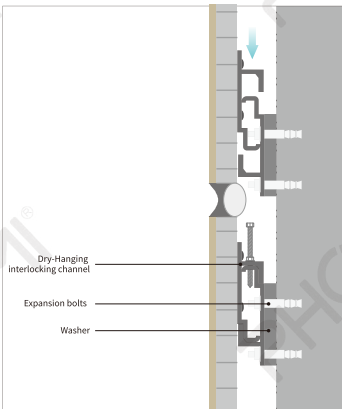
Schematic diagram of Dry-Hanging
