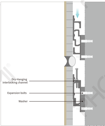
Schematic diagram of Dry-Hanging
