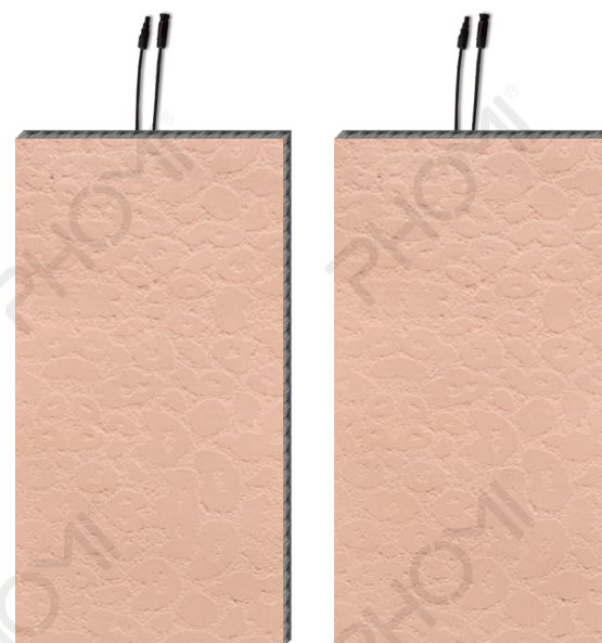
e-solarfacade Butterfly Stone OnO2 1140mmX570mm 50W/m 2 -120W /m 2
